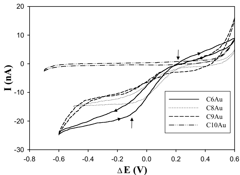
Fig. 4. I - V curves of varied nanoparticle monolayers with the interparticle distance ( L ) roughly equal to a single chainlength of the corresponding protecting monolayer. Potential scan rate 10 mV/s. Arrows indicate the current onsets.
