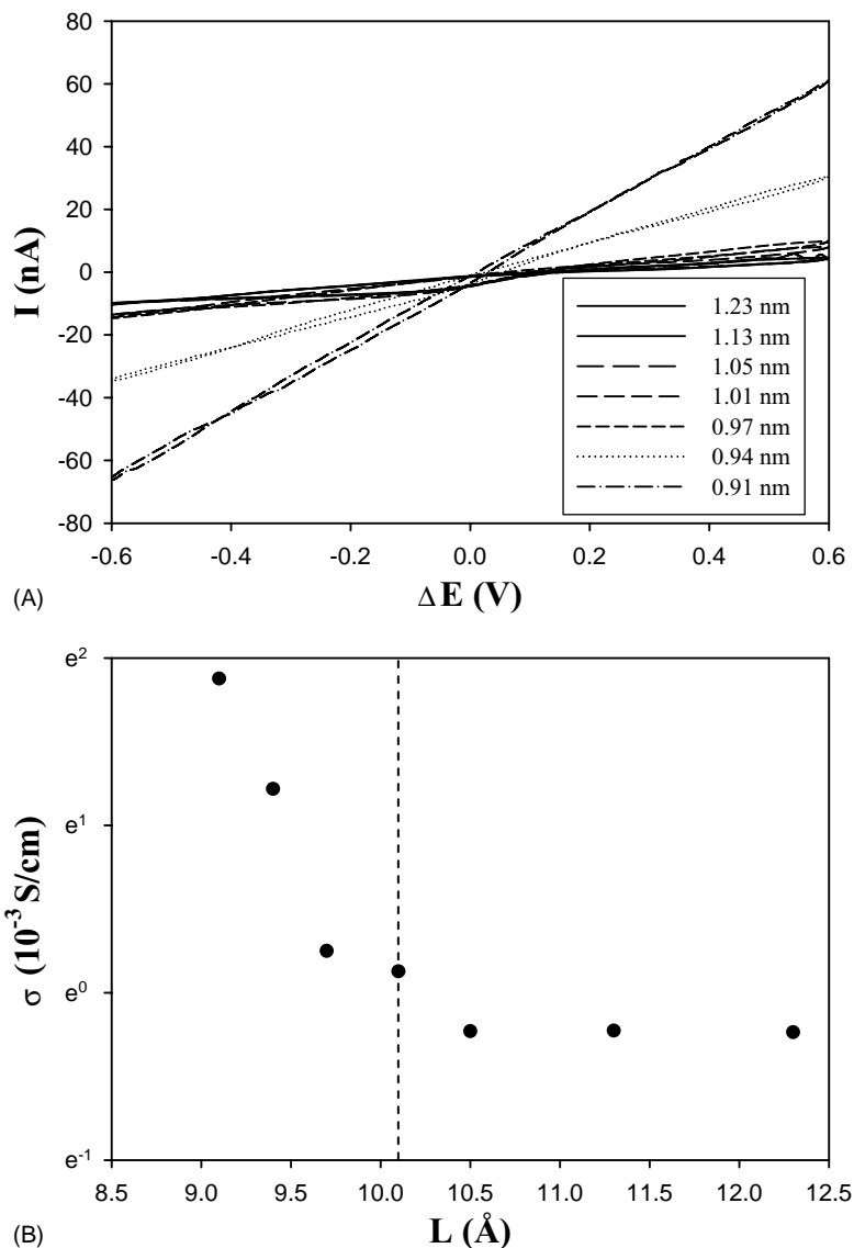
Fig. 3. I - V curves of C5Au nanoparticle monolayers at varied edge-to-edge interparticle distances ( L ) which were shown in figure legends. Potential scan rate 10 mV/s. (B) Variation of electronic conductivity with the interparticle spacings.
