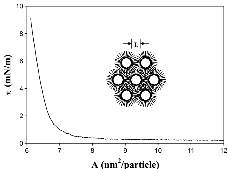
Fig. 1. Surface pressure ( \pi )–area ( A ) isotherm of the Langmuir monolayer of n -butanethiolate-protected gold (C4Au) nanoparticles (diameter 2 nm). Inset shows the schematic particle assemblies on the water surface ( L denotes the edge-to-edge distance between neighboring particles).
