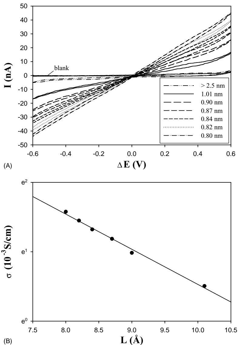
Fig. 2. (A) I - V curves of C4Au nanoparticle monolayers at varied edge-to-edge interparticle distances ( L ) which were shown in figure legends. Potential scan rates 10 mV/s. (B) Variation of electronic conductivity with the interparticle spacings. Symbols are experimental data and line is the linear regression.
