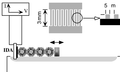
Scheme 1. Schematic setup of the electrical conductivity measurements of nanoparticle Langmuir monolayers. Inset shows the dimensions of the interdigitated array (IDA) electrode.
