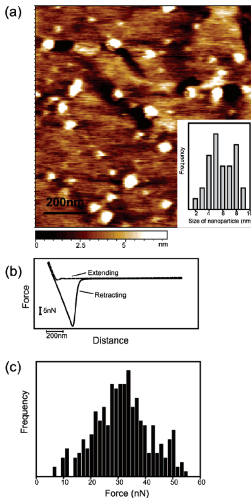
Figure 2. (a) Representative AFM image of Janus particles on the C6 SAM-modified Au(111) surface acquired in tapping mode, scan rate 2.3 lines/s. Inset shows the size distribution of the Janus particles. (b) Typical force–distance curve and (c) histogram of the adhesion force between the tip and the Janus particles on C6 SAM-modified Au(111).
