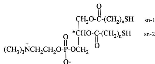
Scheme 1. Chemical Structure of \omega -Thiolated Phospholipids
