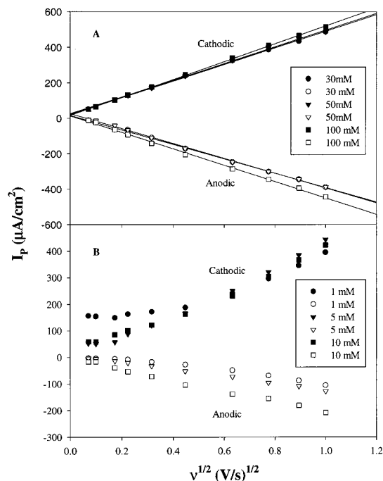
Figure 4. Variation of K_3Fe(CN)_6 anodic and cathodic peak currents with potential sweep rate at various Ca^{2+} concentrations: (A) 30, 50, and 100 mM; (B) 1, 5, and 10 mM. Experimental conditions the same as in Figure 3. Lines shown in (A) are linear regressions.
