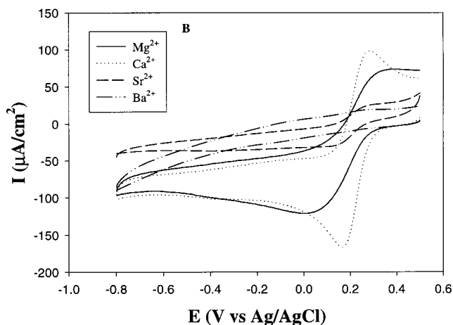
Figure 3. (A) Cyclic voltammograms of a PC-2C11SH SAM-modified gold electrode in 0.1 M NaCl (pH = 7.93 buffered by 0.01 M Tris-HCl) with 1 mM \text{K}_3\text{Fe}(\text{CN})_6 and varied concentration of \text{Ca}^{2+} (no \text{Ca}^{2+} was added with the bare electrode). (B) Cyclic voltammograms of the lipid-modified electrodes in the same electrolyte solutions containing varied divalent ions. The divalent ion concentrations were all 30 mM. Potential sweep rates in (A) and (B) all at 100 mV/s.
