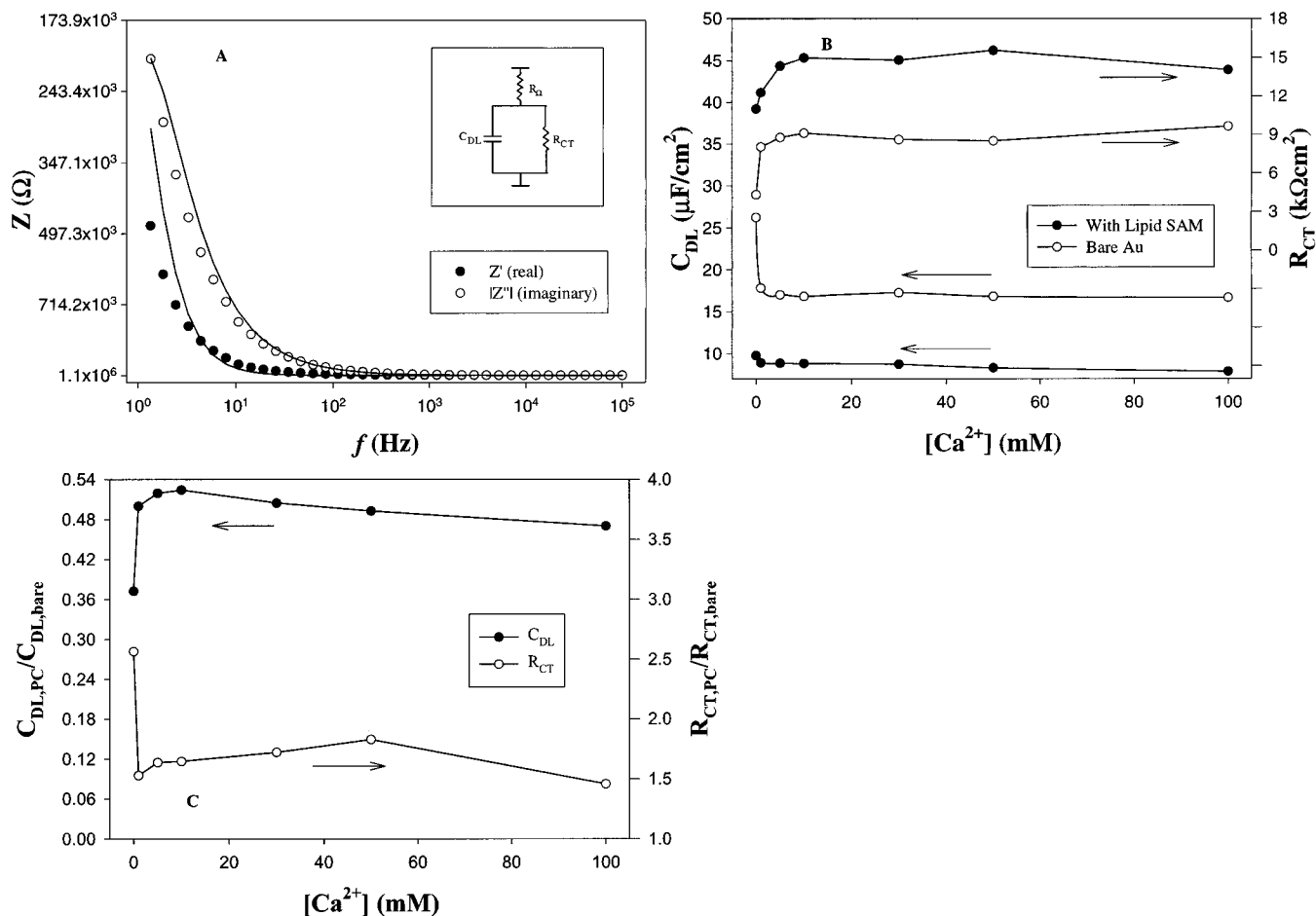
Figure 2. (A) Representative impedance spectra (symbols) of a lipid-modified electrode (conditions same as in Figure 1) at [Ca^{2+}] = 5 mM. Frequency range from 1 to 100 kHz, ac amplitude 10 mV, dc potential bias -0.2 V. The spectra were fitted (solid lines) by the equivalent circuit shown in the inset. (B) Variation of electrode interfacial capacitance ( C_{DL} ) and charge-transfer resistance ( R_{CT} ) with Ca^{2+} concentration which were determined from (A). (C) Variations of the ratios of C_{DL} and R_{CT} in the presence and absence of lipid adlayers with Ca^{2+} concentration.
