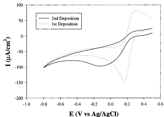
Figure 5. Cyclic voltammograms of a PC-2C11SH SAM-modified gold electrode in 0.1 M NaCl (pH = 7.93 buffered by 0.01 M Tris-HCl) with 1 mM K_3Fe(CN)_6 and 50 mM Ca^{2+} . The electrode was pretreated in 50 mM Ca^{2+} followed by immersion into the lipid solution for additional deposition (—); also shown is the CV with the first lipid assembly (---, from Figure 3). Potential sweep rate 50 mV/s.
