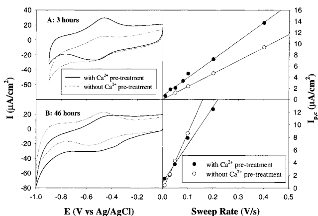
Figure 6. Cyclic voltammograms of the lipid-modified electrodes that were incubated into viologen thiol-derivative solution for a second deposition for (A) 3 h and (B) 46 h, with and without a pretreatment of 100 mM \text{Ca}^{2+} (left panels). Sweep rate 200 mV/s. The right panels show the corresponding variation of peak current with sweep rate (symbols) fitted with the linear regressions (solid lines).
